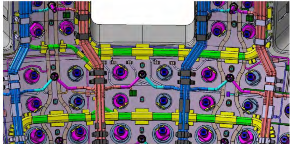
Figure 7.3-8 – Completed Outboard Circuit Blankets 16C-16S
